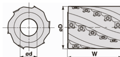
Drawing
